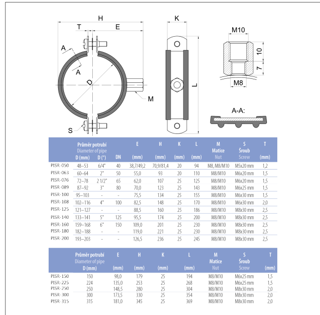
PISR - Dimension sketch
