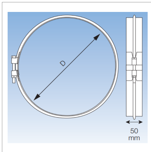
PRTD- wide pull ring
